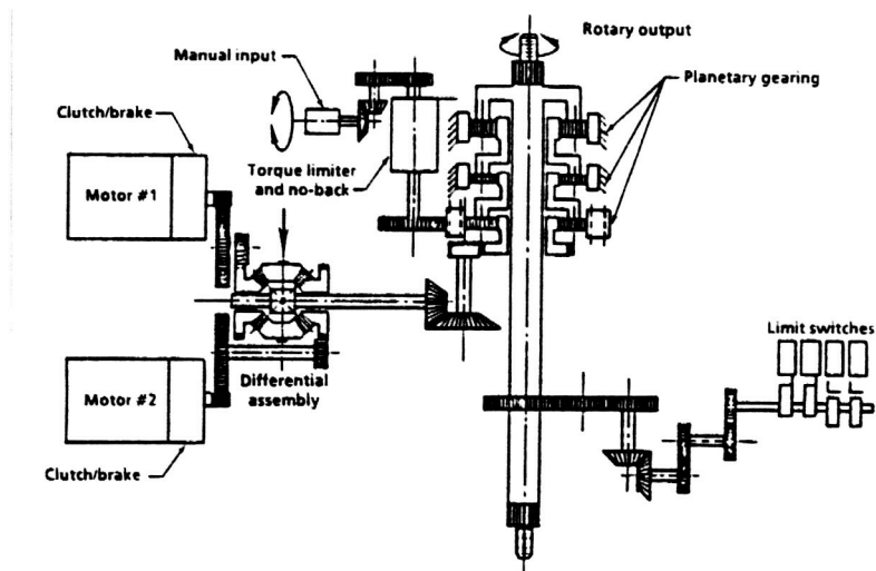
PLBD Centerline Latch Actuator Schematic
